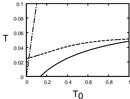
Fig. 2. Case 2. \alpha = 0.4 . AT-line(solid curve) and the zero-entropy line(dashed curve) in space of (T_0, T) .
