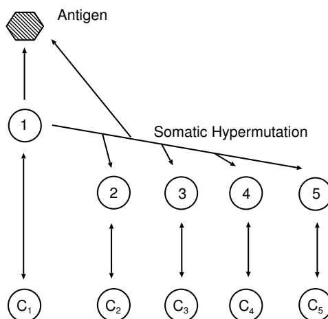
FIGURE 13. Explanation of model 3 in which antibodies and anti-idiotypic antibodies are taken into account.
