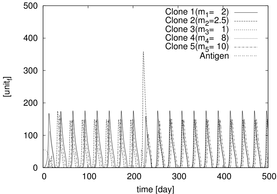
FIGURE 15. Time series of concentrations of antibodies f_i for model 3. A_0 = 55 [unit f ], A'_0 = 55 [unit f ]. Timing of second invasion is different from that in Fig. 10.
